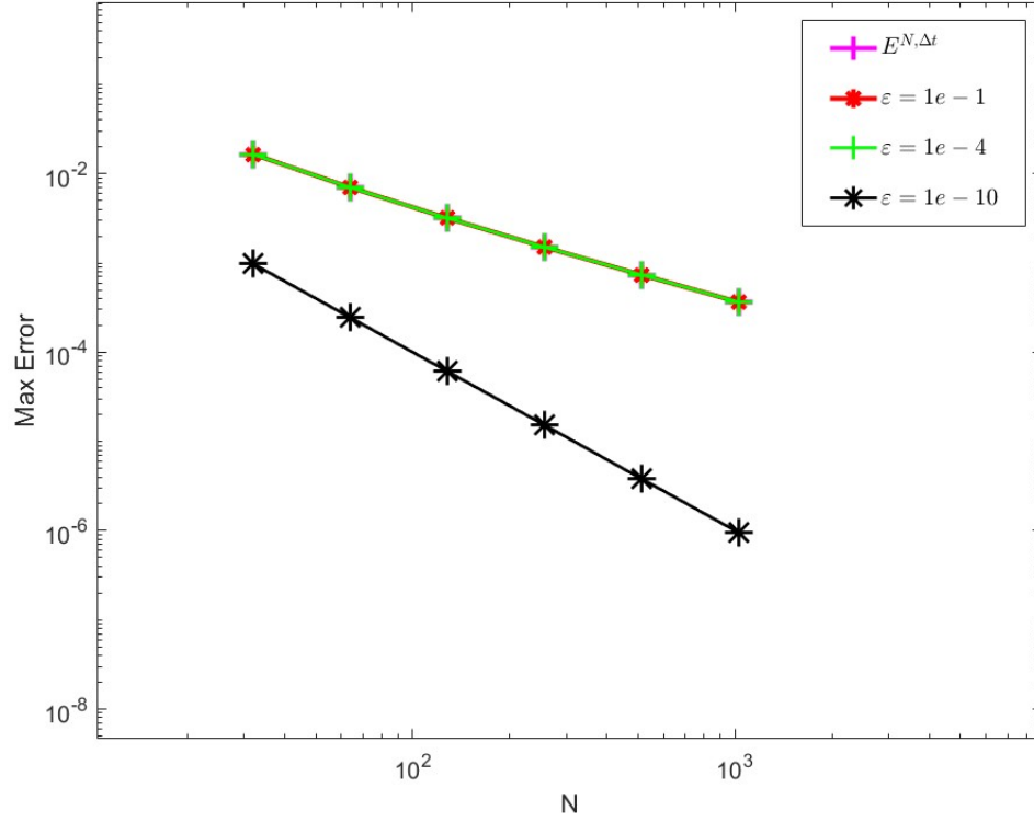
Figure 1: Loglog plot of the maximum point-wise error obtained by the numerical scheme (3.14) using Example 6.2
