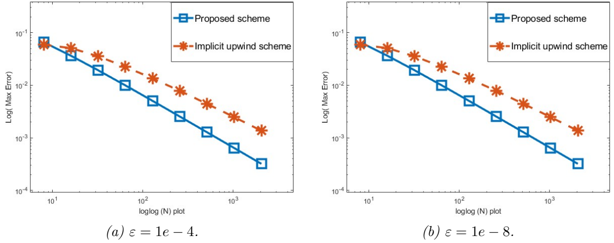
Figure 2: Loglog plot for comparison of the error to the solution (3.1.1) using numerical scheme (3.33) and (3.58)
