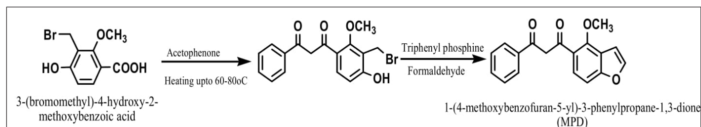
Figure 1. Process map for synthesis of MPD.
