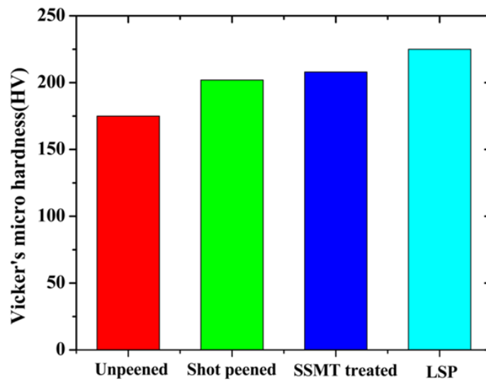
Fig. 1 Surface hardness plot
